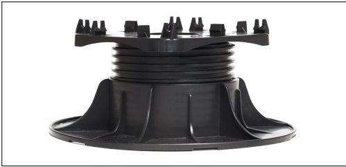
Self-Levelling Adjustable Joist Support Pedestal with Clip-on Head RDA-C
